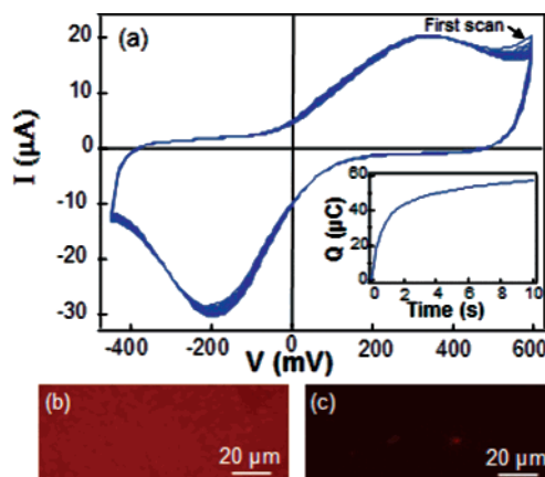
Figure 2. (a) Fifteen consecutive CVs showing the reversible oxidation/reduction of a SAM of HQ-PA on an ITO glass sheet. (Inset) Chronoamperometry shows the amount of charge necessary to oxidize a predefined area of HQ-PA: an average of 56.8 μC. (b) A fluorescence image of ITO surface that was oxidized to Q-PA, reacted with SH-DNA, and the DNA paired to its complementary DNA strand labeled with a fluorescence dye. (c) A fluorescence image of ITO with the HQ-PA monolayer went through the same DNA attachment procedure as that of the ITO sheet in (b), showing little or no DNA binding.
