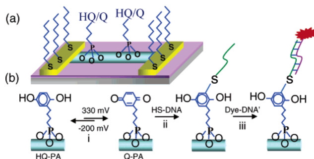
Figure 1. (a) Schematic representation of an In 2 O 3 NW mat device (only one NW is shown for clarity). The NW is functionalized with a SAM of HQ-PA and is placed between two gold electrodes protected by a SAM of dodecane-1-thiol. (b) (i) The monolayer of HQ-PA, deposited on the In 2 O 3 NW or ITO, can be reversibly oxidized to Q-PA in an electrochemical cell. (ii) Addition of the probe, thiol-terminated DNA (HS-DNA) to Q-PA. (iii) Attachment of complementary DNA strand (dye-DNA') to the probe DNA.
