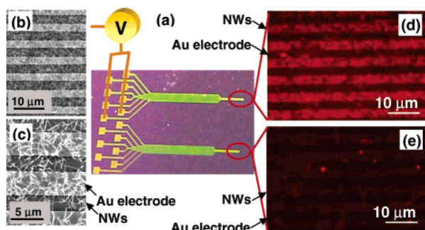
Figure 3. (a) A photograph of a NW mat sample contacted by two groups of electrodes. Only the HQ-PA attached to the NWs between the upper electrodes was converted to Q-PA. (b) An SEM image of the \text{In}_2\text{O}_3 NWs before functionalization. The brighter stripes are gold electrodes covering the NW mat. (c) The same sample imaged at higher magnification, where the NW mat is clearly visible. (d) A fluorescence image of the NWs with Q-PA taken after DNA attachment. The gold electrodes, passivated with an alkanethiol, appear dark under the fluorescence microscope. (e) A fluorescence image of the NWs with HQ-PA after DNA incubation. The NWs appear dark, indicating no DNA attached to HQ-PA.
